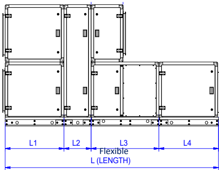
STACKED AHU
