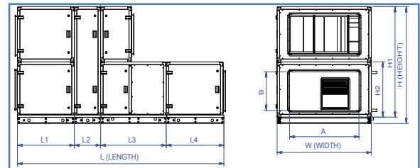
STACKED AHU
